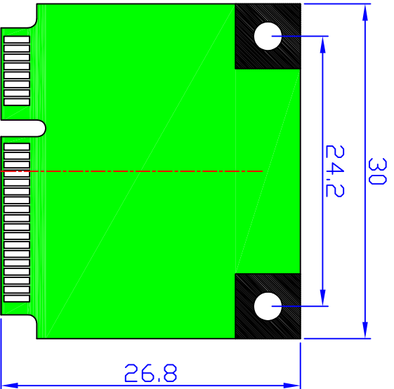
Half-Mini Card dimension
